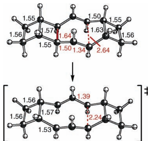
FIGURE 1. Reactant and transition-state structures for the [3,3] sigmatropic shift in a broken [6]-ladderane [B3LYP/6-31G(d)]. Selected distances are shown in angstroms. 4
