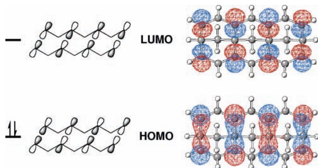
FIGURE 3. Delocalized molecular orbitals [B3LYP/6-31G(d)] for a singlet \sigma -polyene. 10
