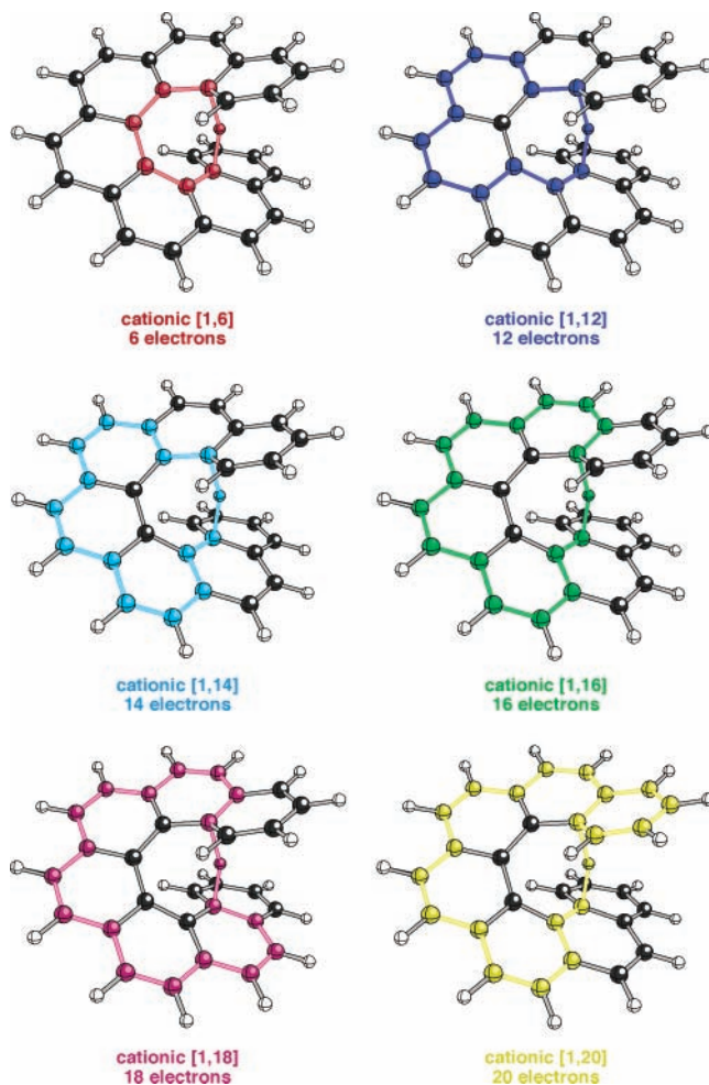
FIGURE 12. Various \pi circuits present in the transition structure shown in Figure 11.
