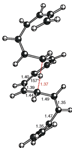
FIGURE 5. Transition structure [B3LYP/6-31G(d)] for a model of the [1,7] shiftamer shown in Scheme 6 (distances shown in angstroms). 13
