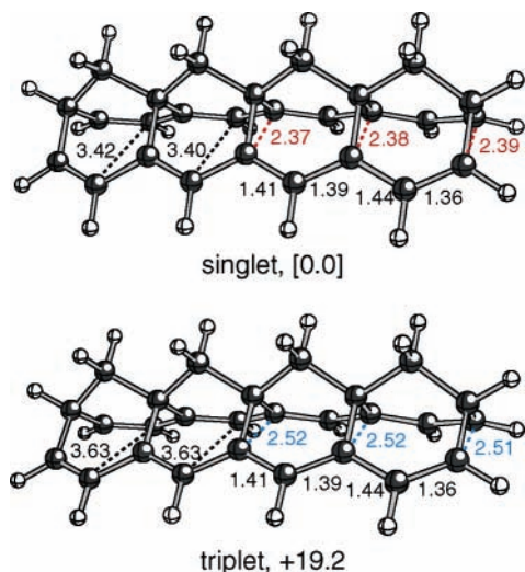
FIGURE 2. Geometries (selected distances shown in angstroms) and relative energies (kcal/mol) of fully optimized singlet and triplet models of the proposed shiftamer shown in Scheme 5 [B3LYP/6-31G(d)]. 10
