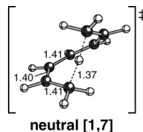
FIGURE 4. Transition structure for the [1,7] sigmatropic shift of heptatriene [B3LYP/6-31G(d); distances shown in angstroms]. 2b,13
