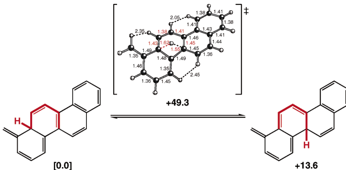
FIGURE 9. [1,5] Shift (highlighted in red) in a model of the top system shown in Chart 4, studied at the B3LYP/6-31G(d) level (selected distances are shown in angstroms, and relative energies are shown in kcal/mol). 15
