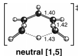
FIGURE 8. Transition structure for the neutral [1,5] shift of 1,3-pentadiene (selected distances are shown in angstroms). 2b
