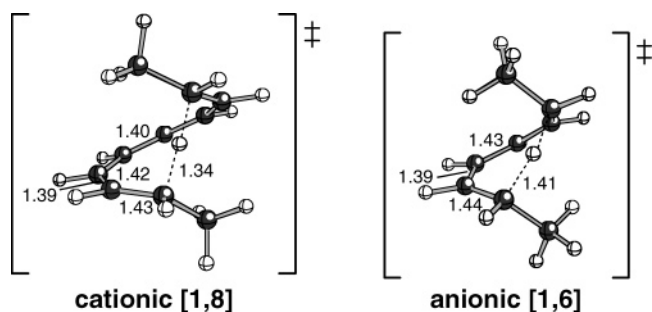
FIGURE 7. Transition structures for dimethyl-substituted cationic [1,8] and anionic [1,6] rearrangements (selected distances are shown in angstroms). 13b
