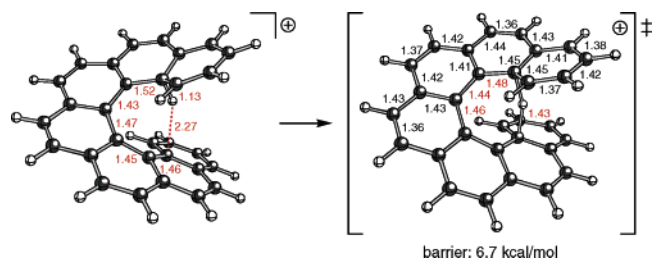
FIGURE 11. Protonated 7 and the transition structure for its antarafacial [1,6] hydrogen shift (selected distances are shown in angstroms).
