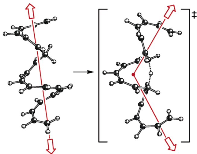
FIGURE 6. Different view of the transition structure shown in Figure 5 and its precursor. The reorientation of the hydrocarbon chain as the reaction proceeds is emphasized by the red lines and arrows.
