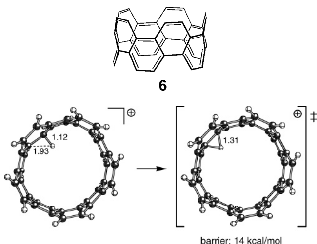
FIGURE 10. "In-protonated" 6 and the transition structure for its [1,2] hydrogen shift (selected distances are shown in angstroms). 15
